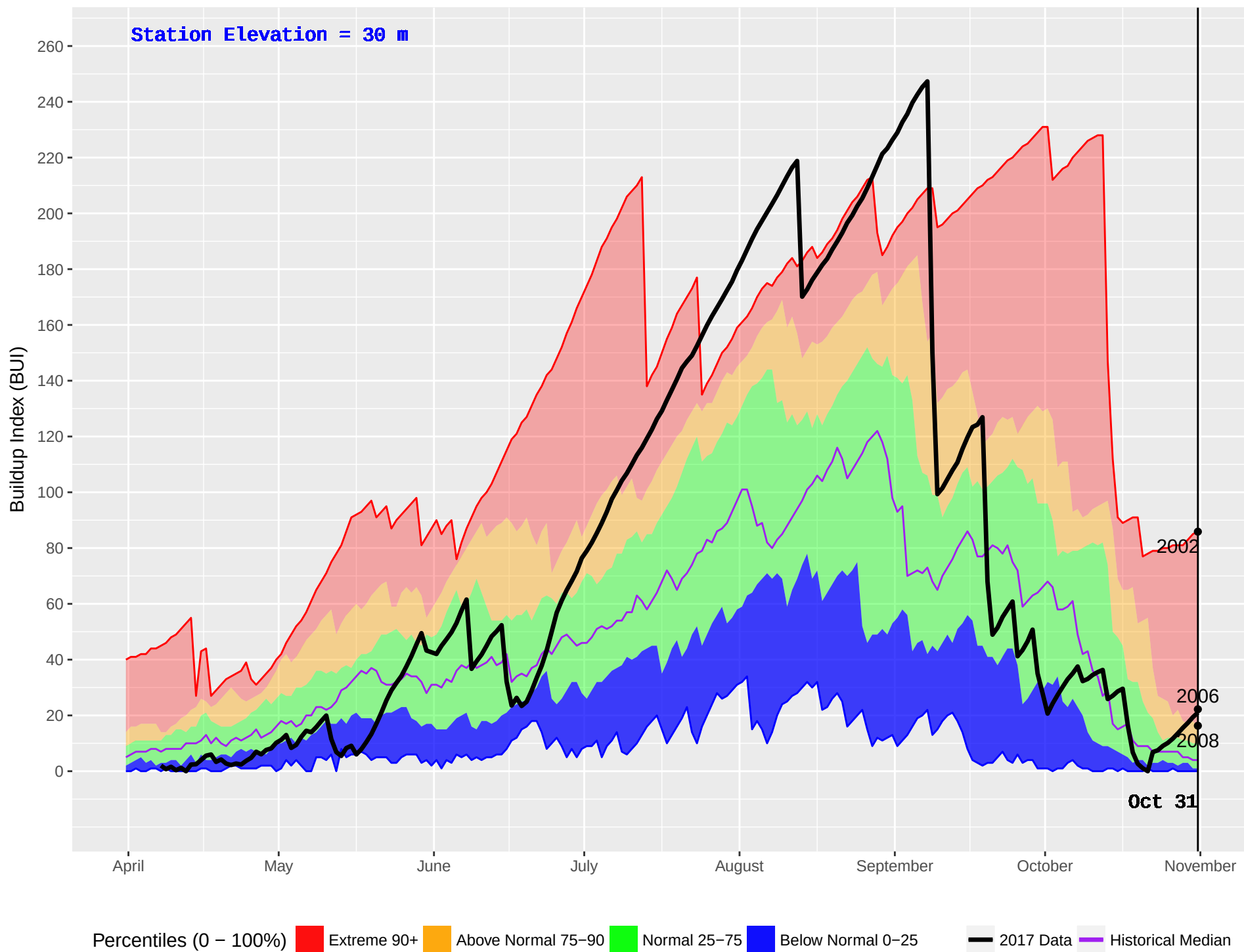
CEDAR (59) : Historical (1989–2016) and Current (2017) Noon Buildup Index (BUI)
