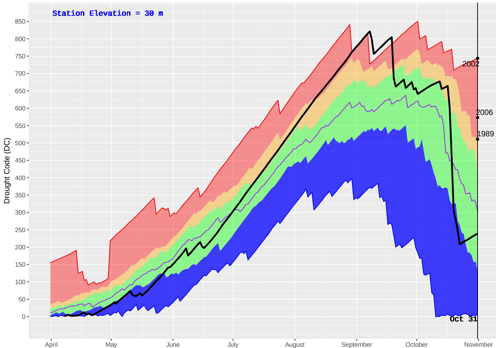
CEDAR (59) : Historical (1989–2016) and Current (2017) Noon Drought Code (DC)
