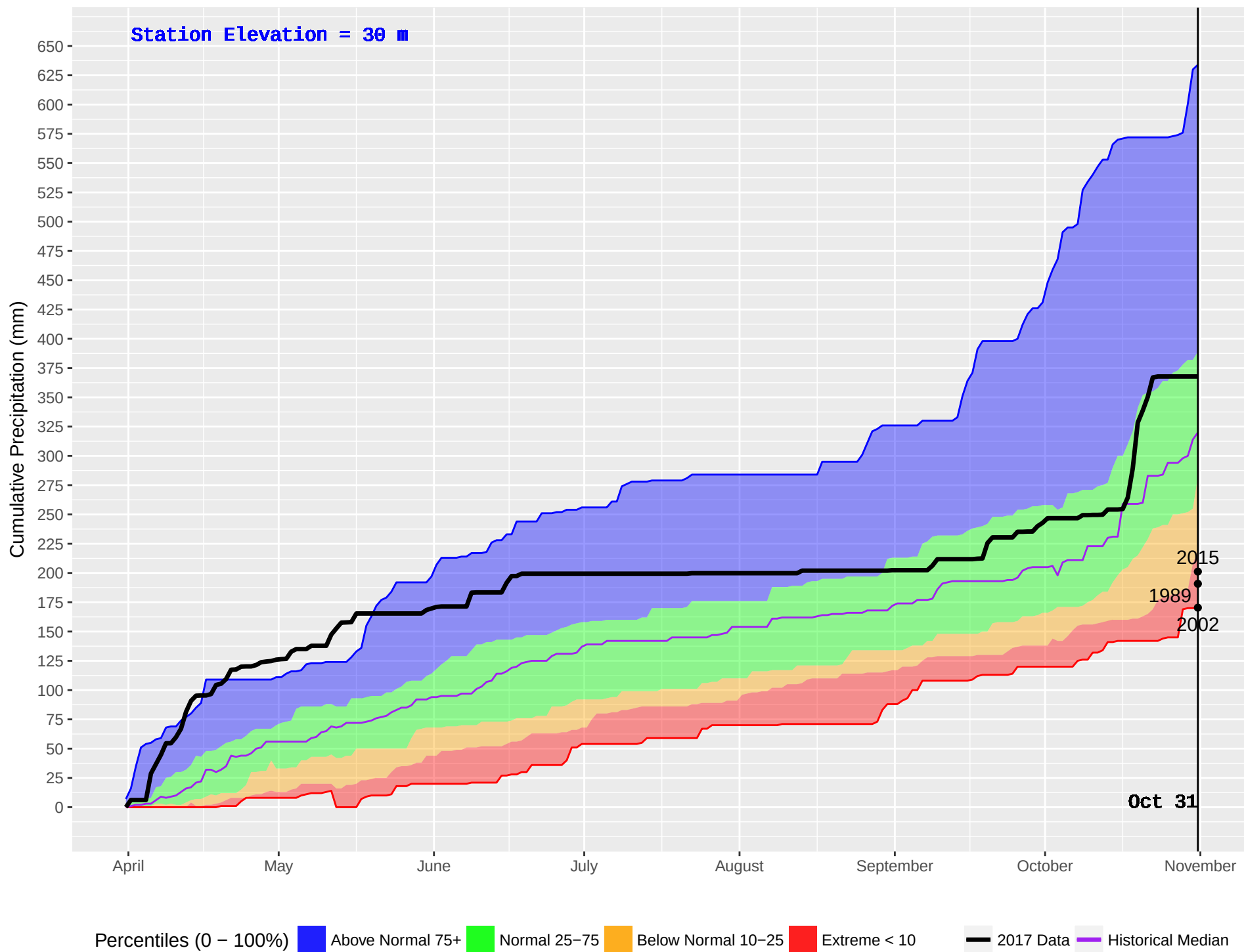
CEDAR (59) : Historical (1989–2016) and Current (2017) Noon Cumulative Precipitation
